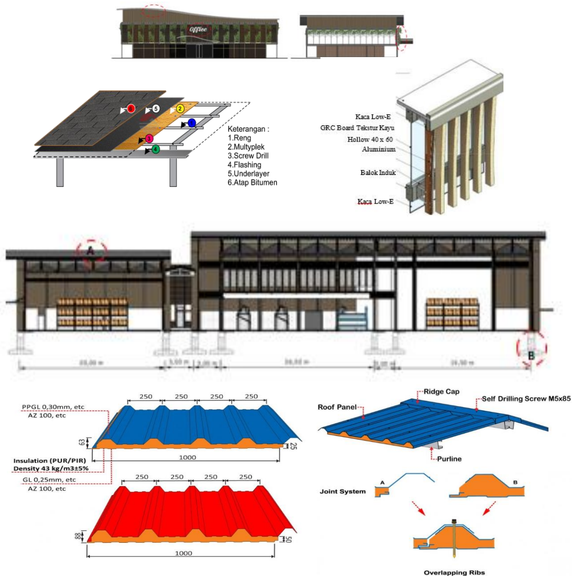
Gambar 10. Detail Material
