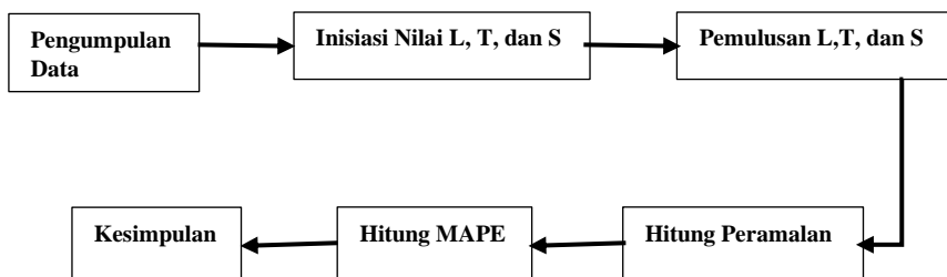
Gambar 1. Metode Penelitian
