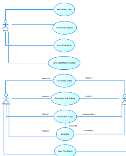
Gambar 2. Diagram Use Case Sistem
