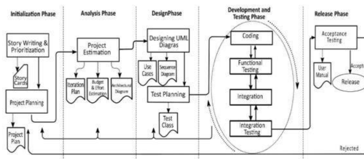
Gambar 1. Alur proses model Extreme Programming
