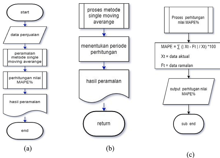
Gambar 2. a) Flowchart Sistem Peramalan, b) Flowchart Metode, c) Flowchart MAPE%.
