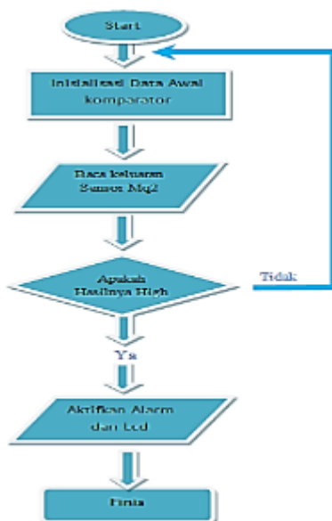
Gambar 4. Flowchart Sistem
