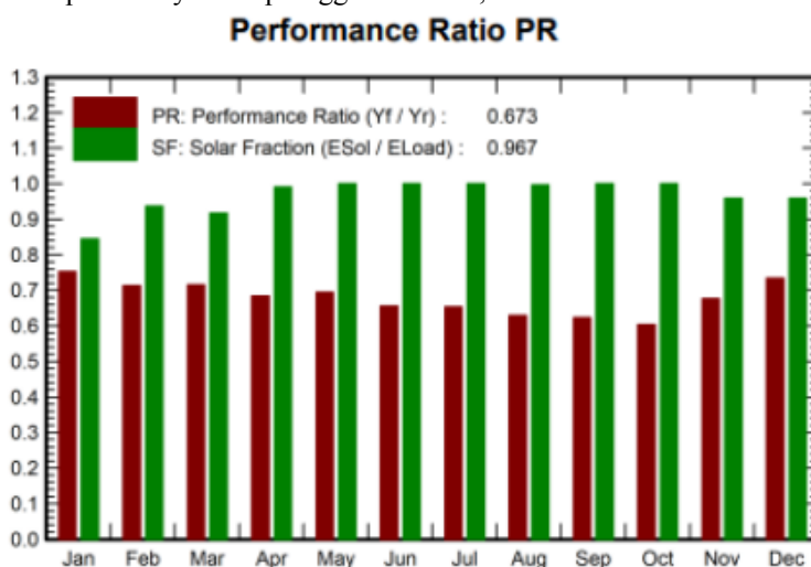
Gambar 4. Performance Ratio
