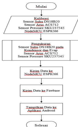
Gambar 4. Flowchart Sistem
