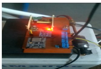
Gambar 3. Hardware Sistem Monitoring AC Berbasis IoT
