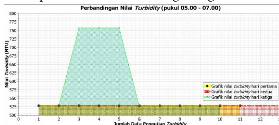
Gambar 10. grafik nilai Turbidity pukul 05.00 – 07.00
