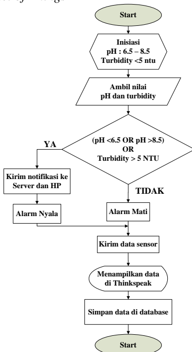
Gambar 2. Flowchart system
