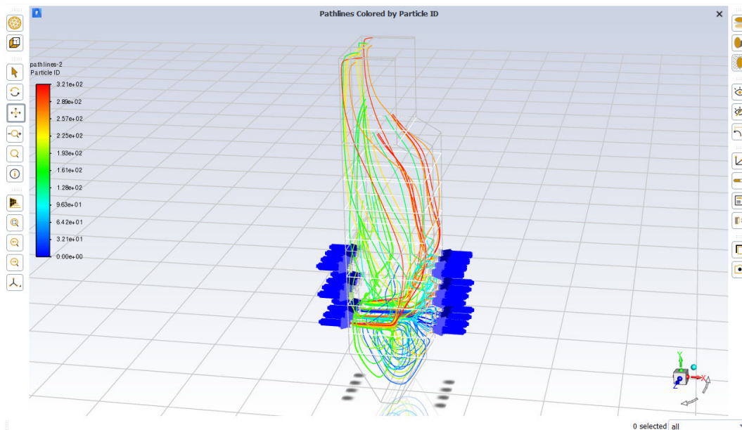
Gambar 7. Particle pathlines burner A
