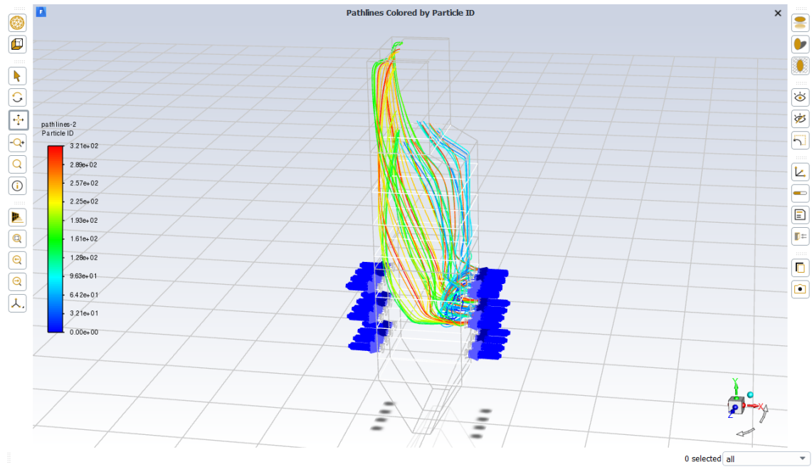
Gambar 11. Particle pathlines burner E
