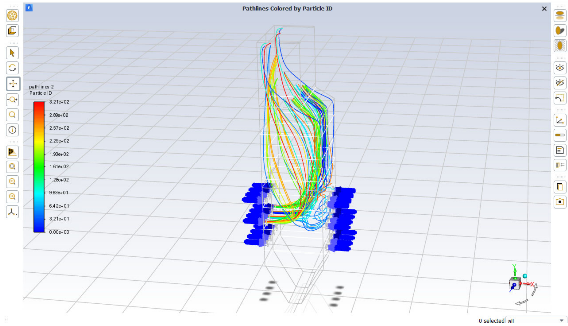
Gambar 8. Particle pathlines burner B
