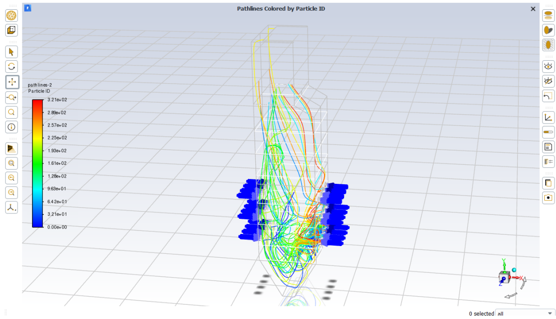
Gambar 10. Particle pathlines burner D
