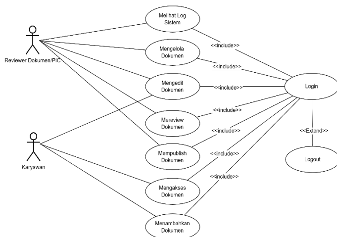
Gambar 2. Usecase Diagram
