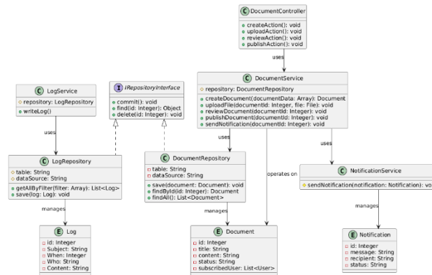
Gambar 6. Class Diagram
