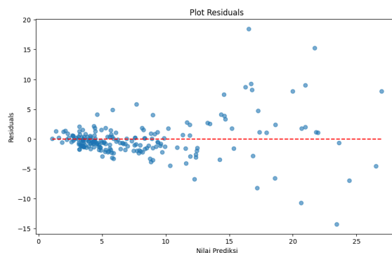
Gambar 3. Plot Residuals
