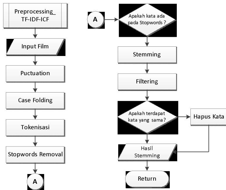
Gambar 2. Flowchart sub proses Preprocessing
