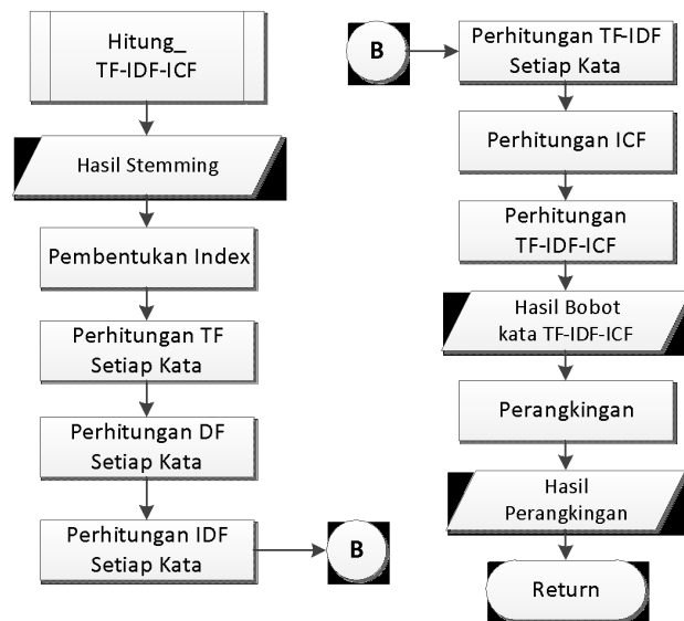
Gambar 3. Flowchart sub proses Hitung TF-IDF-ICF
