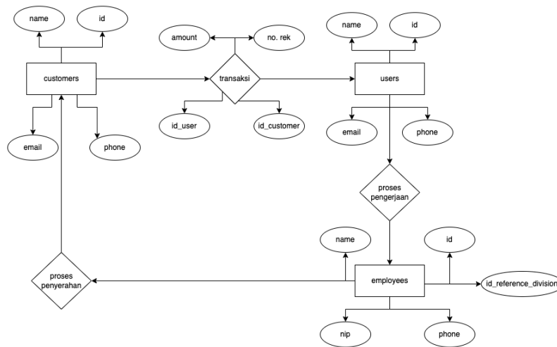
Gambar 6 Entity Relationship Diagram
