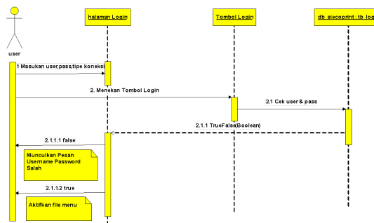
Gambar 1 Sequence Diagram
