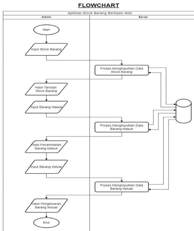
Gambar 1. Flowchart
