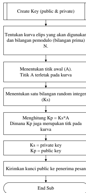
Gambar 4. Flowchart Create Key Algoritma Elliptic Curve Cryptography (ECC)
