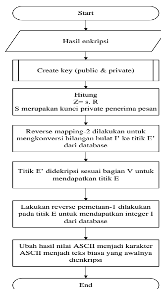
Gambar 3. Flowchart Dekripsi Algoritma ECC
