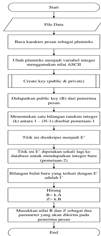
Gambar 2. Flowchart Enkripsi Algoritma ECC
