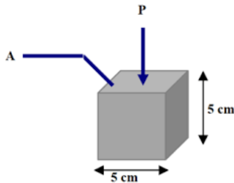
Gambar 2. Detail Benda Uji Penelitian
