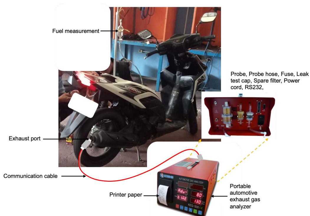
Figure 1. Experimental setup
