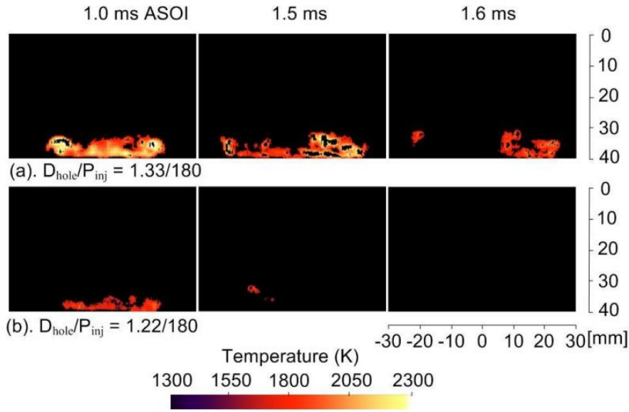
Figure 7. Comparison of temperature distribution at 0.122 and 0.133 mm nozzle hole diameter under an injection pressure of 180 MPa.
