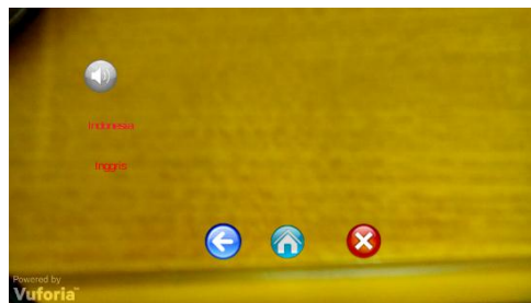
Gambar 8. Scene AR
