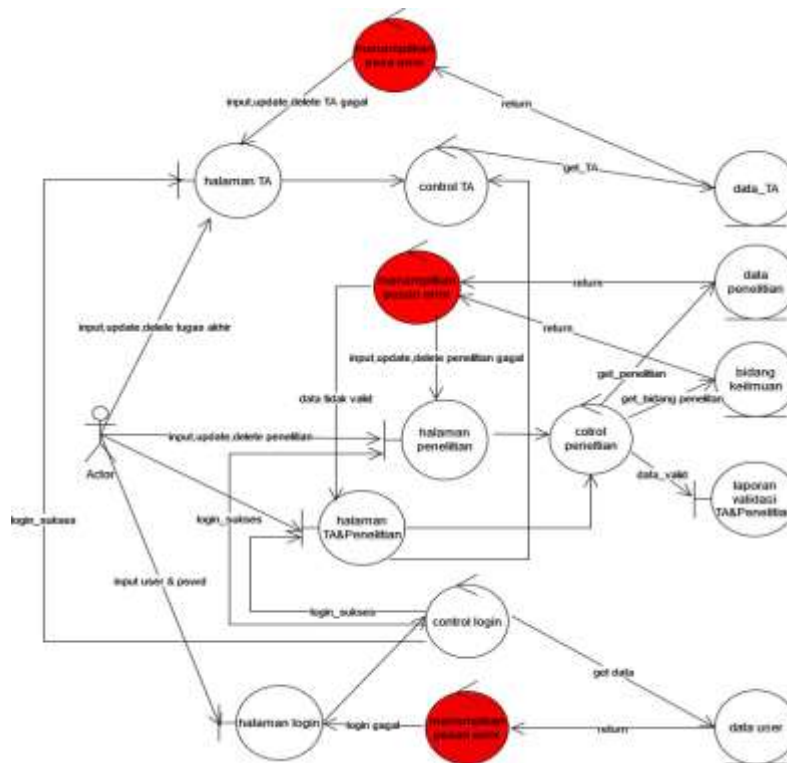
Gambar 4. Robustness diagram
