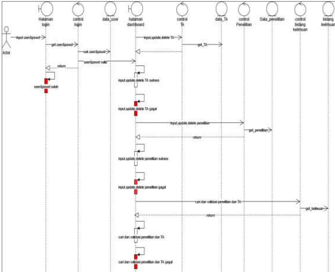
Gambar 5. Sequence diagram
